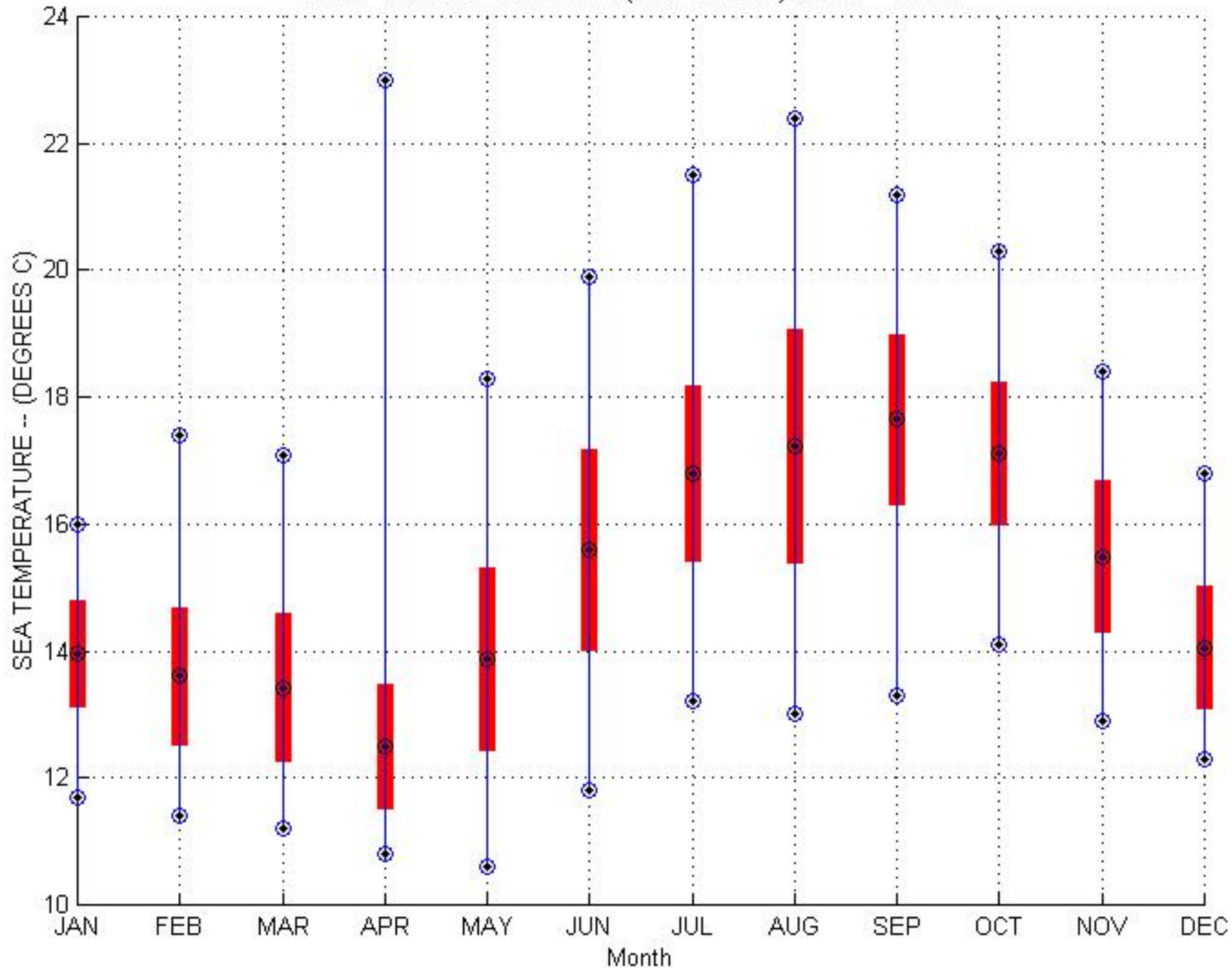
46053 SEA TEMPERATURE ( DEGREES C) 1/1994 - 12/2001
